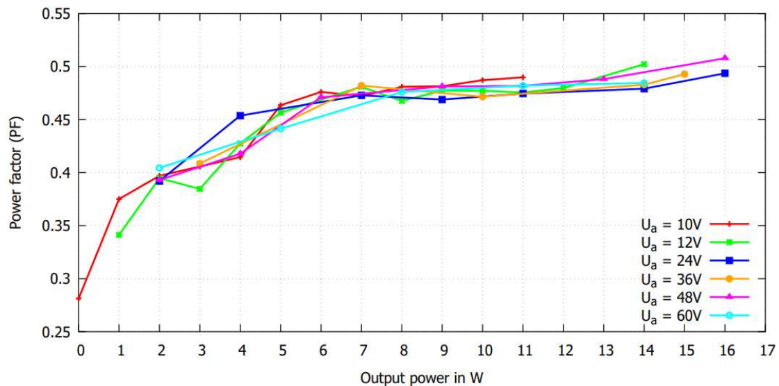
Figure 9: Power factor as a function of electrical power
