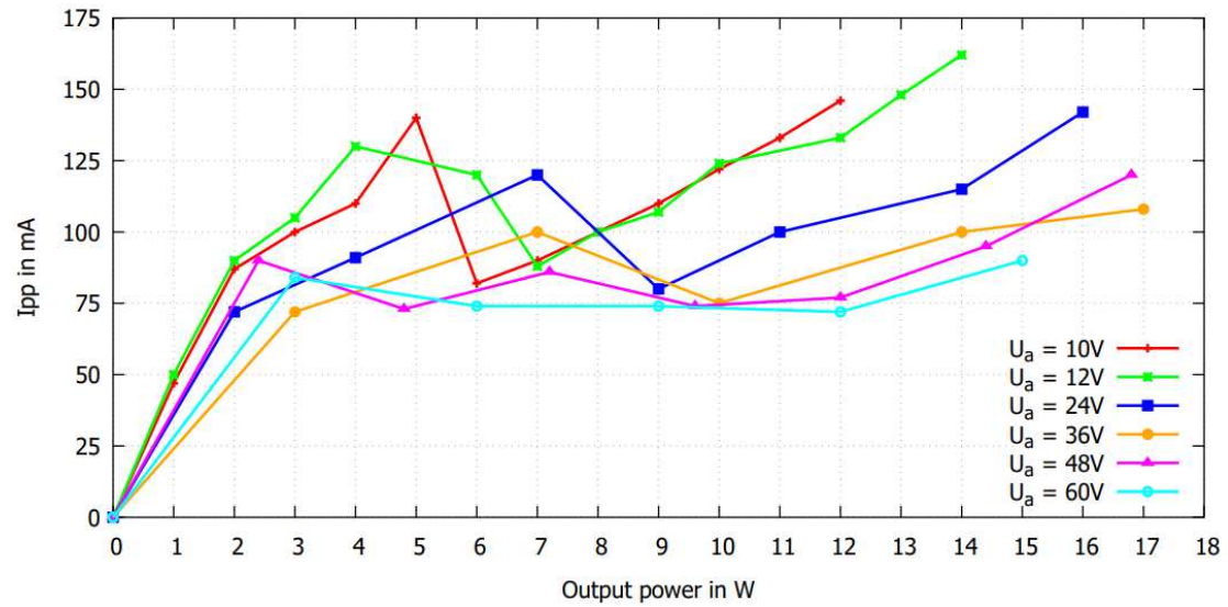
Figure 10: Peak-to-peak current as a function of electrical power
