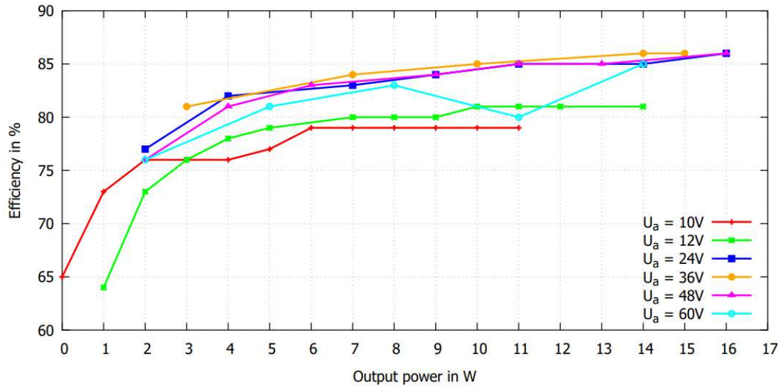
Figure 8: Efficiency as a function of electrical power
