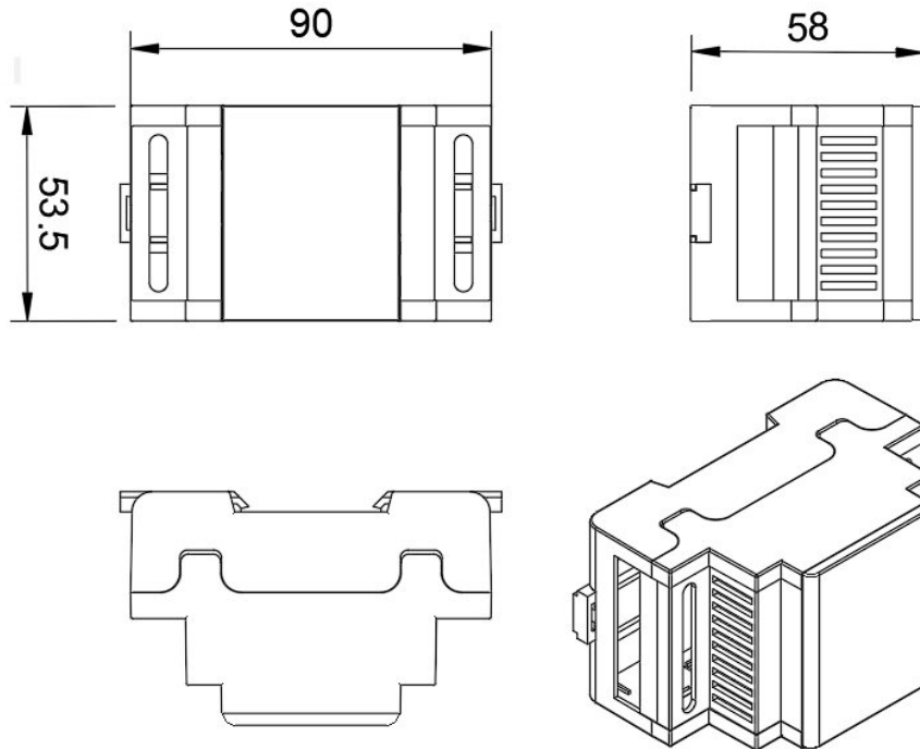
Figure 13: DIG-CCCV-15W Product case.
