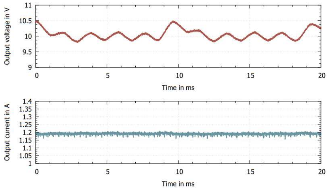
Figure 6: Full-Load behavior at 10V output voltage and 1.2A output current
