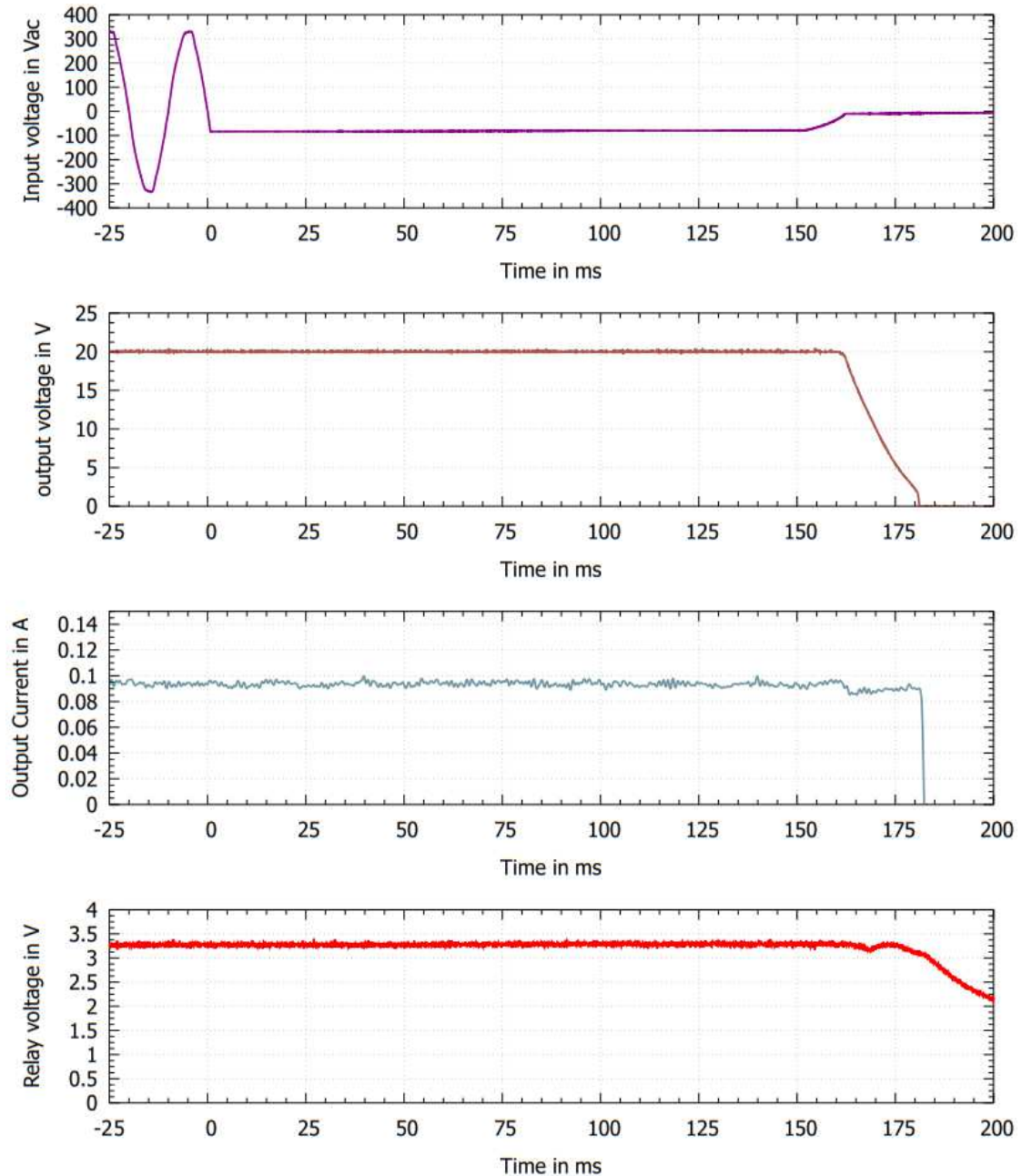
Figure 3: Switch off behavior for 20V output voltage and 0.1A output current
