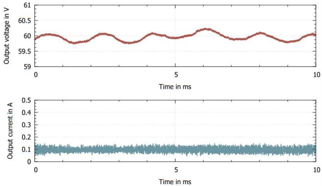
Figure 7: Full-Load behavior at 60V output voltage and 0.1A output current
