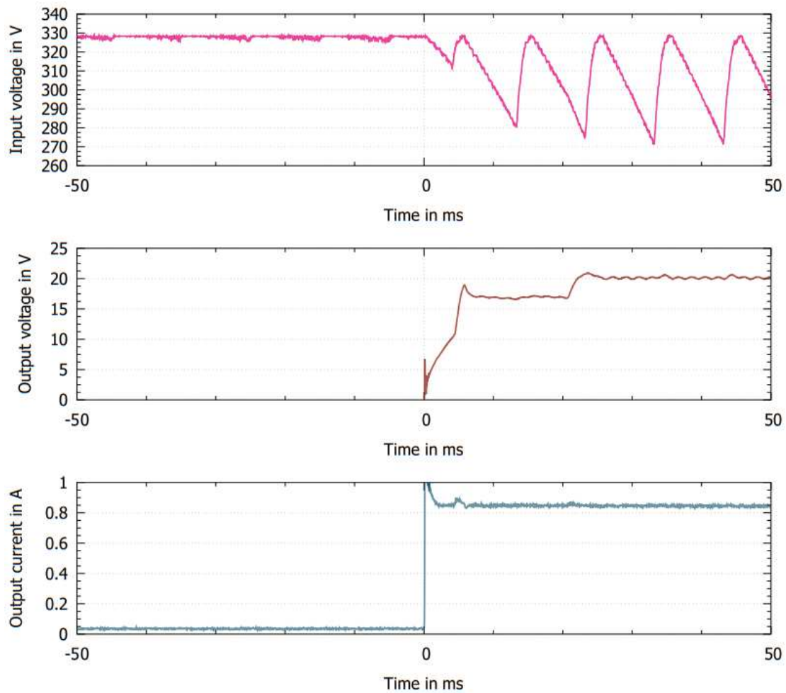
Figure 4: Load on behavior for 20V output voltage and 0.84A output current
