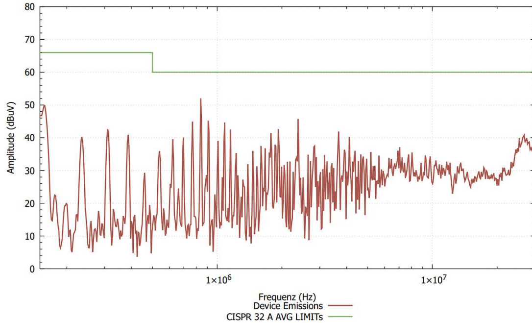
Figure 11: Conducted Input emissions
