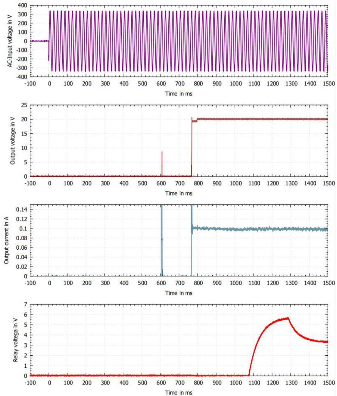
Figure 2: Switch on behavior for 20V output voltage and 0.1A output current
