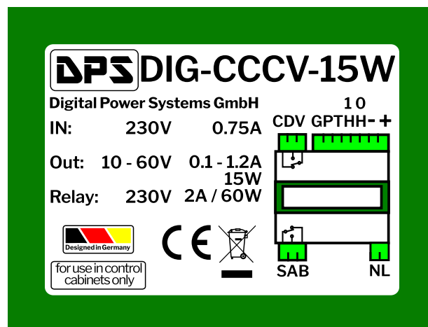
Figure 14: The product label of the DIG-CCCV-15W.
