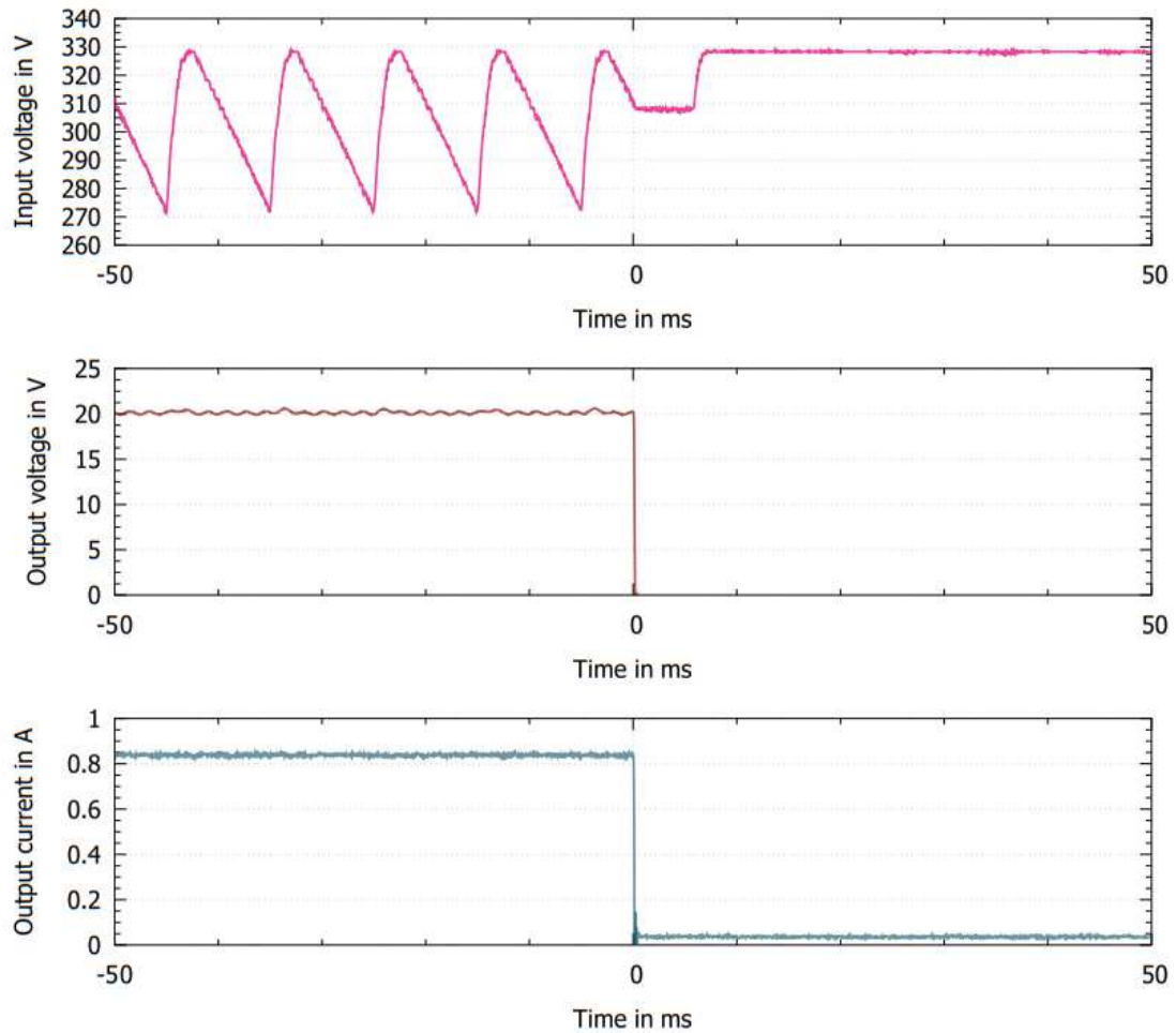
Figure 5: Load off behavior for 20V output voltage and 0.84A output current
